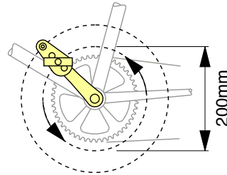
Crank Shortener: position C
